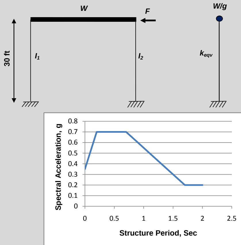
Design Response Spectrum
